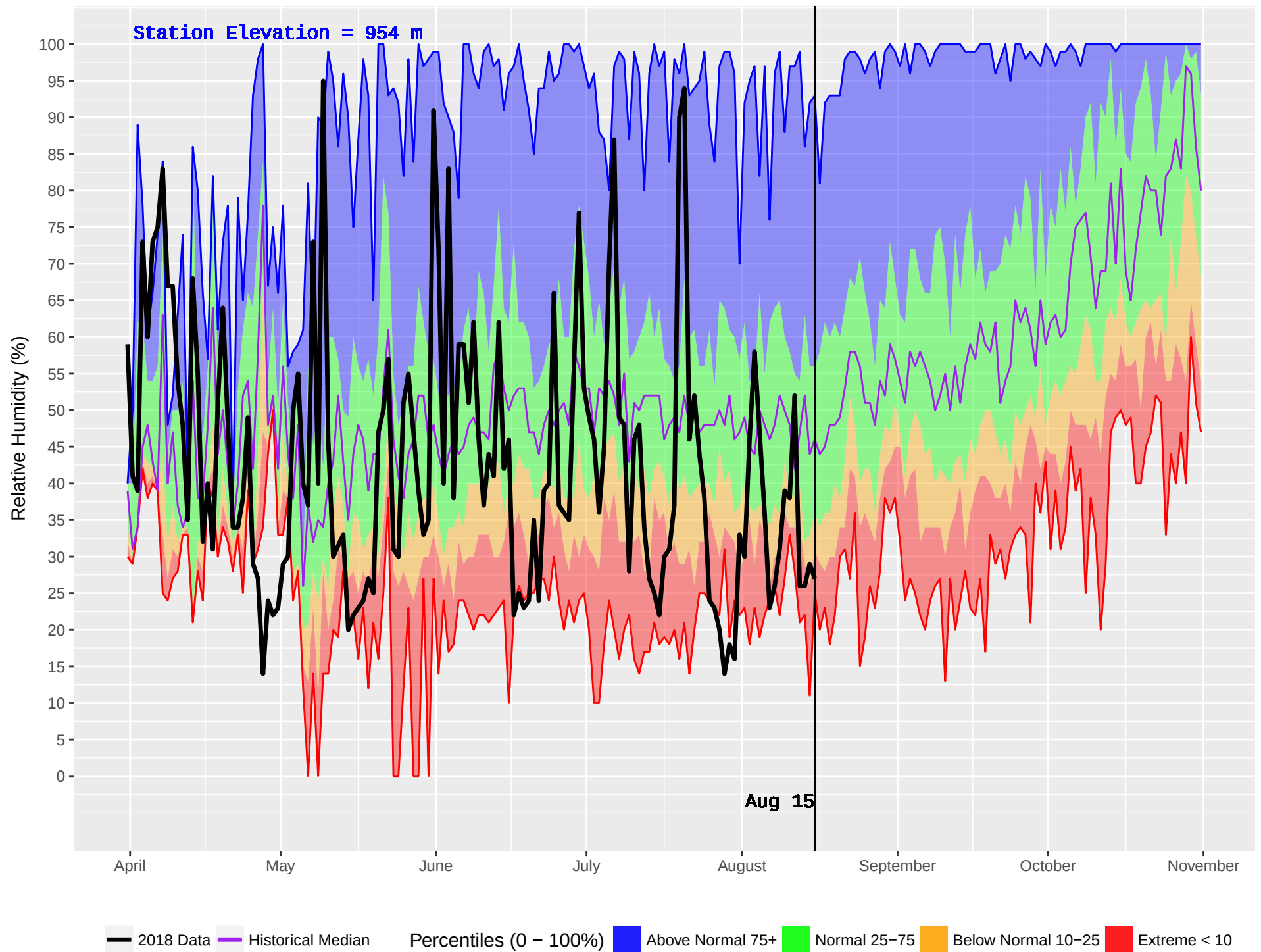
NADINA (179) : Historical (1985–2016) and Current (2018) Daily Relative Humidity
