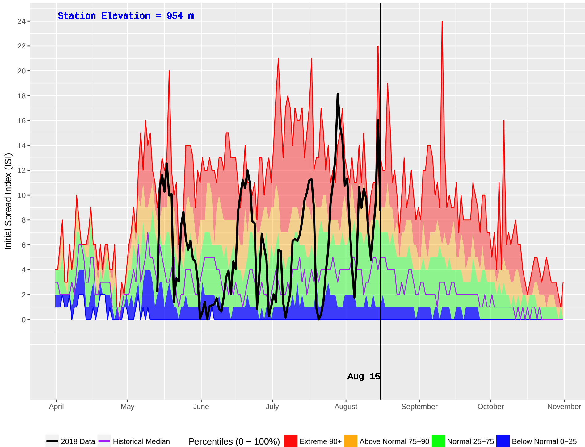
NADINA (179) : Historical (1985–2016) and Current (2018) Daily Initial Spread Index (ISI)
