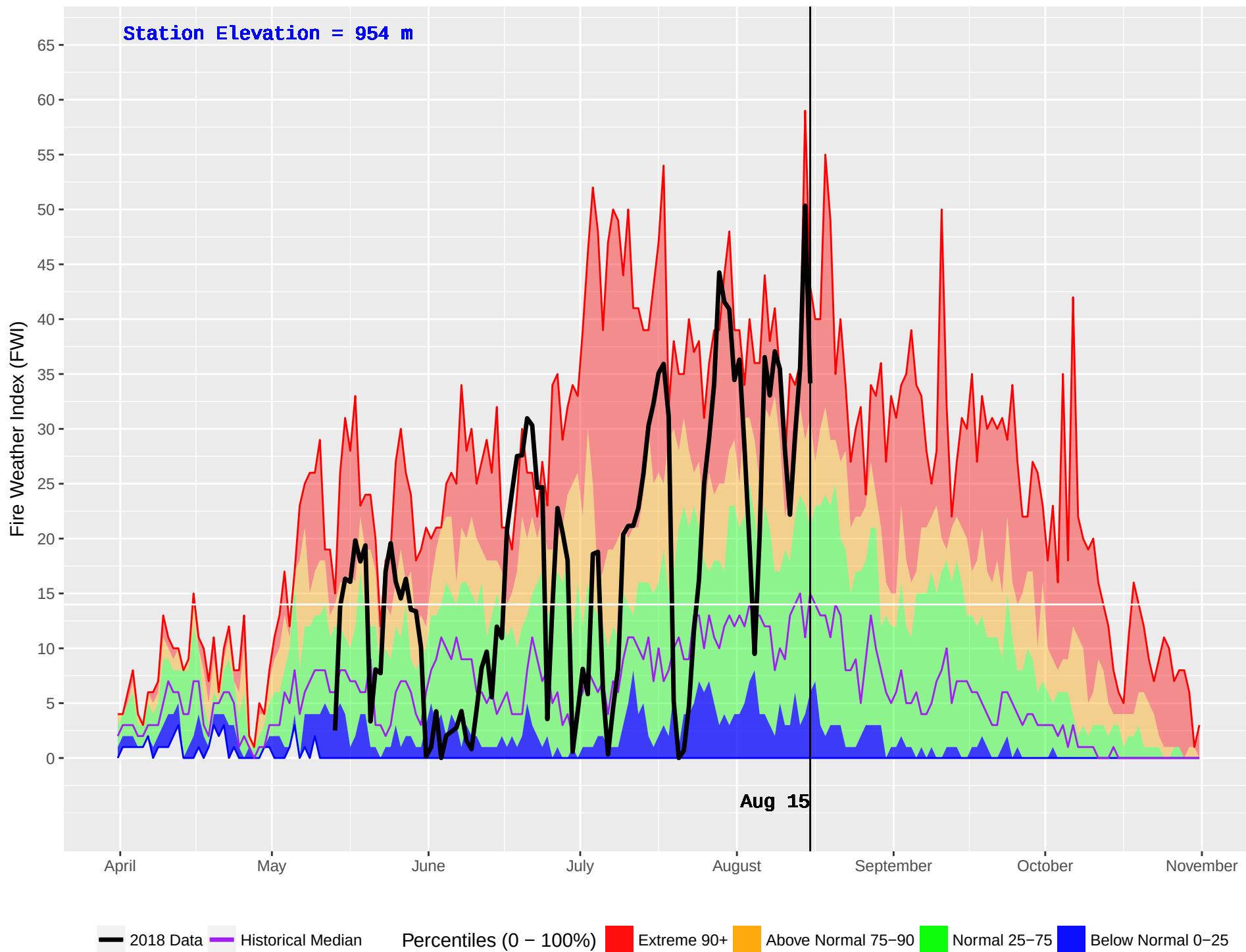
NADINA (179) : Historical (1985–2016) and Current (2018) Daily Fire Weather Index (FWI)
