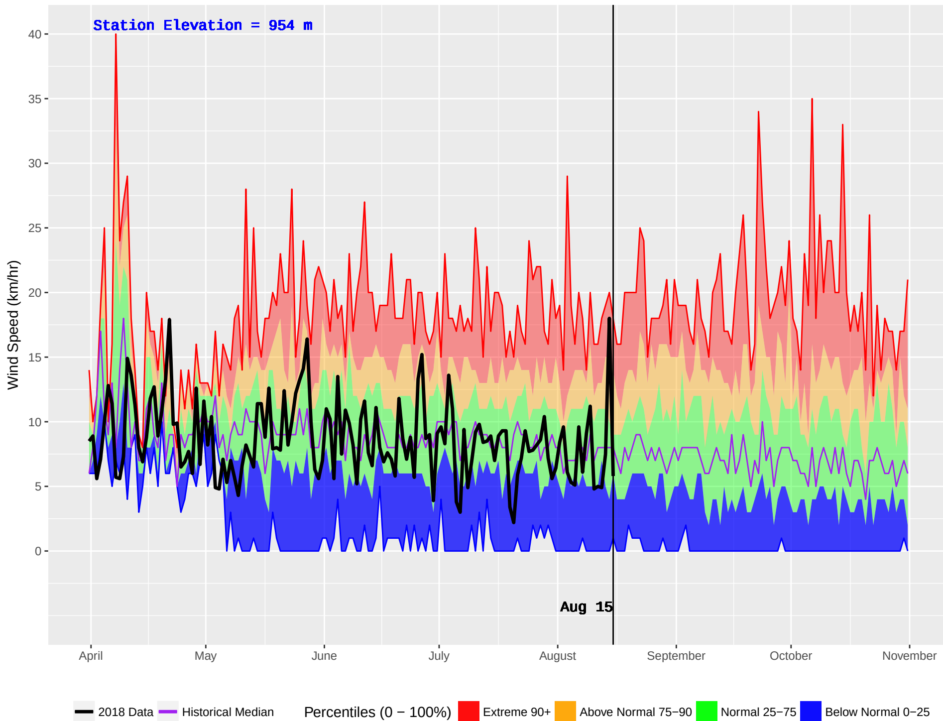
NADINA (179) : Historical (1985–2016) and Current (2018) Daily Wind Speed
