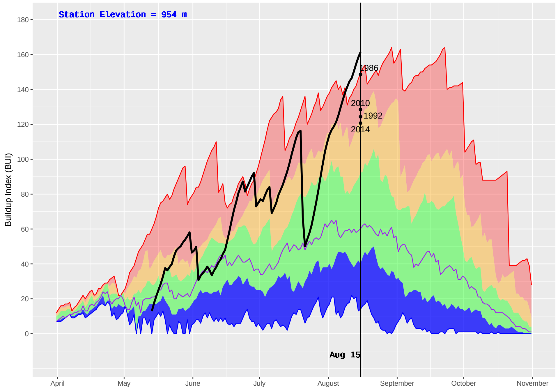
NADINA (179) : Historical (1985–2016) and Current (2018) Daily Buildup Index (BUI)
