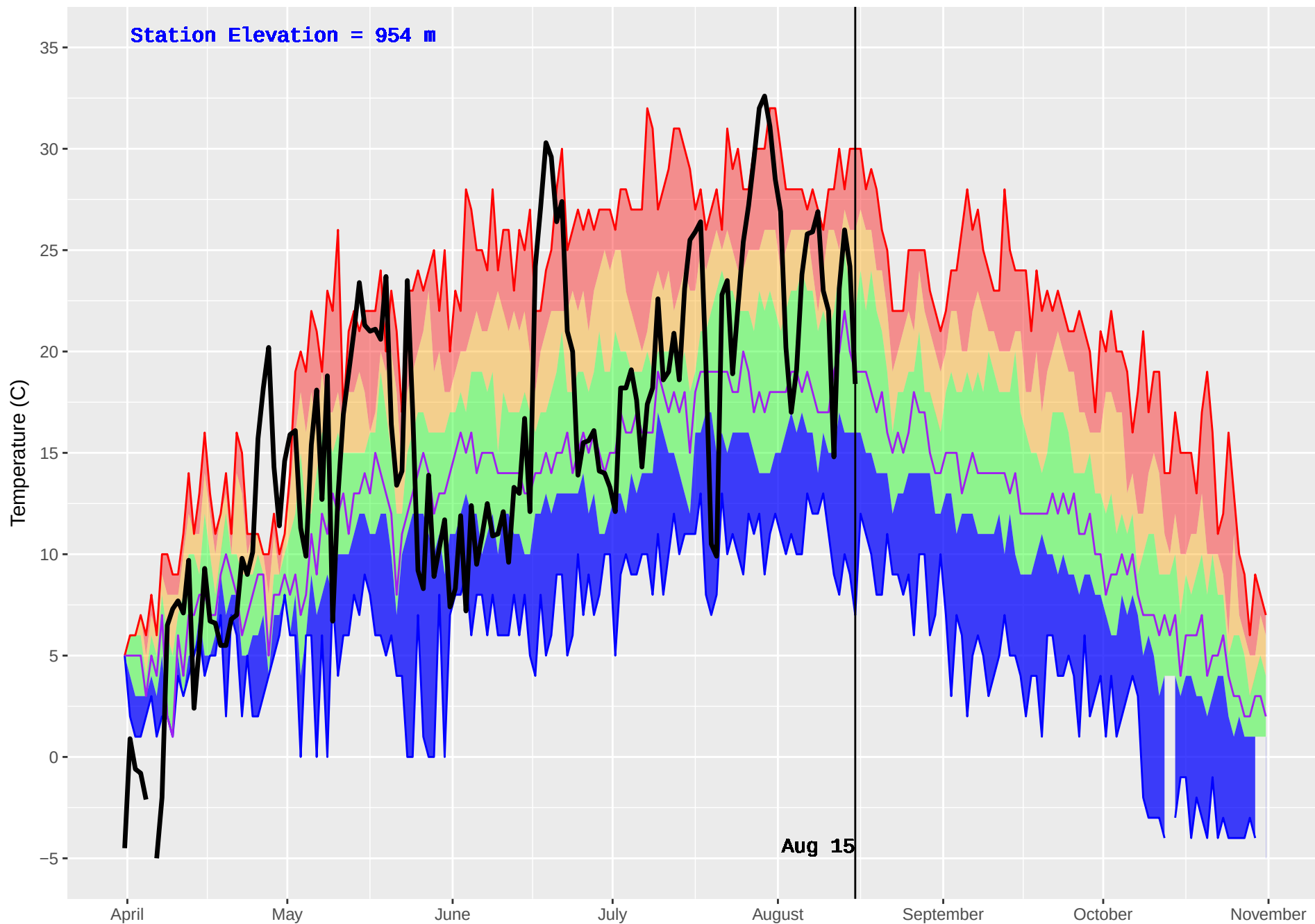
NADINA (179) : Historical (1985–2016) and Current (2018) Daily Temperature
